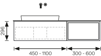
PLI06 1 Ladenelement (Siphon-Lade)* 1 Offenes Element
